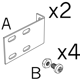
1" Hidden End Mount Extension Bracket and Screws A: PCN 5908071000 (2 Pack) B: PCN 5008068000 (4 Pack)
