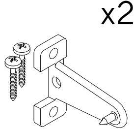
SimpleLift Hold-Down Bracket (Jamb), \frac{3}{4} " KIT2010
