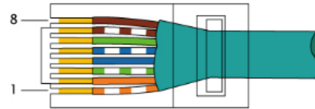
EIA/TIA-568B
