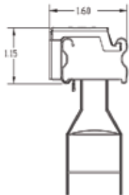
Integrated Bracket Detail
