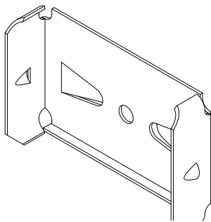
2" Low Profile Headrail End Lock PCN 5003655000
