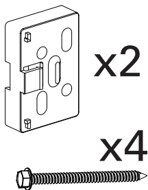
Spacer Block Kits KIT4010
