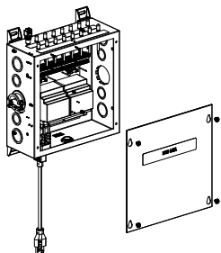
16 Shade DC Power Supply PCN 7810000001
