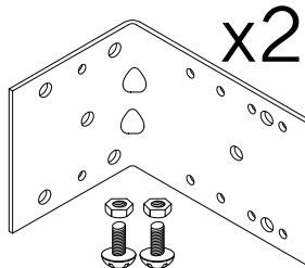
Low Profile Extension Bracket (Short) KIT4380 (2 Pack – Shown) KIT4381 (3 Pack)
