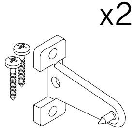
SimpleLift Hold-Down Bracket (Jamb), 3/4" KIT2010
