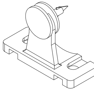
Hold-Down Bracket – Sill/Wall (For Outside Mount Non- Operable Specialty Blinds) PCN 5007313000
