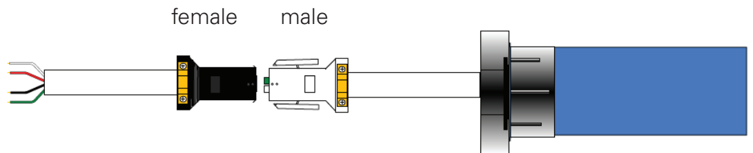
18" White SJWT AWG 18 delivered on motor (4 wire)
