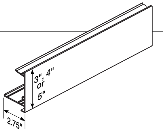
Fig. 1 Standard Fascia Detail
