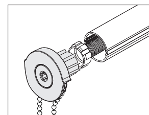
Spring Assist
