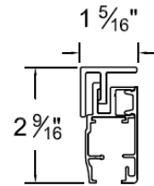
Side Channel Inside Mount
